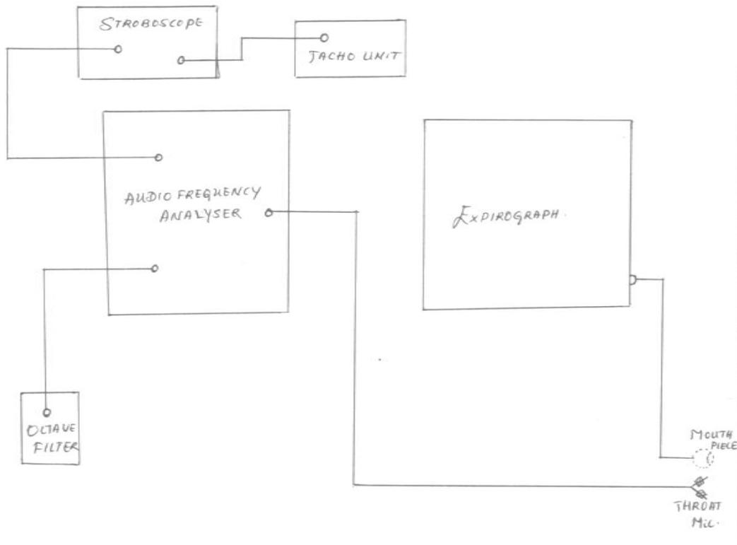
Block Diagram -3
