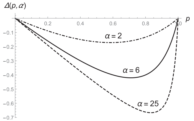
Fig. 3. Reputation losses ( \alpha \in \{2, 6, 25\} ).
