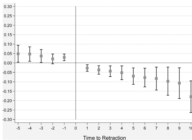
Fig. 8. Dynamics of retraction effect on citations to pre-retraction publications. Note: The dots in the above plot correspond to coefficient estimates stemming from conditional fixed effects quasi-maximum likelihood Poisson specifications in which the citation rates for articles published by retracted and control authors prior to their first associated retraction event are regressed onto year effects, article age indicator variables, as well as 15 interaction terms between treatment status and the number of years before/after the retraction event (the indicator variable for treatment status interacted with the year of retraction is omitted). The 95% confidence intervals (corresponding to robust standard errors, clustered around unique author identifiers) around these estimates is plotted with the help of capped spikes.
