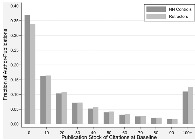
Fig. 6. Cumulative citations to pre-retraction publications. Note: Cumulative number of citations up to the year preceding the corresponding earliest retraction event for 21,103 retracted authors’ publications and 42,115 control authors’ publications.
