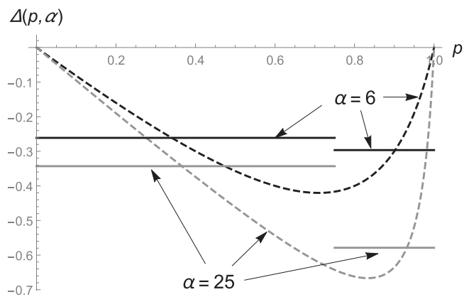
Fig. 4. Average reputation losses ( p^* = 3/4, \alpha \in \{6, 25\} ).
