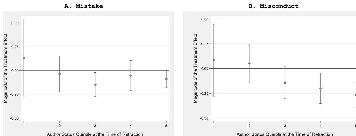
Fig. 9. Retraction effect on citations to pre-retraction publications, by status quintile. Note: The dots in the above plots correspond to coefficient estimates stemming from conditional fixed effects quasi-maximum likelihood Poisson specifications in which the citation rates for articles published by retracted and control authors prior to their first associated retraction event are regressed onto year effects, article age indicator variables, as well as five interaction terms between the treatment indicator variable and five indicator variables corresponding to each quintile of the author status distribution. Status is defined by the author’s cumulative citations at baseline. Panel A limits the sample to publications of retracted authors and their controls who were associated with a retraction event stemming from mistake, while Panel B includes only publications for retracted authors and their controls that were associated with a retraction event stemming from misconduct. The 95% confidence intervals (corresponding to robust standard errors, clustered around unique author identifiers) around these estimates is plotted with the help of capped spikes.
