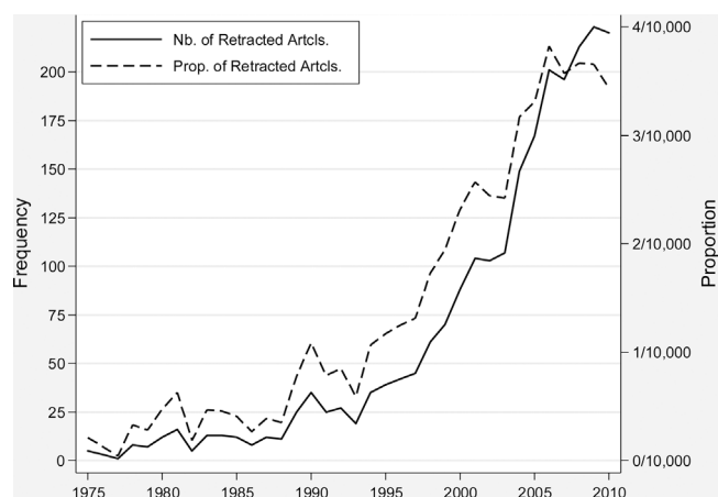
Fig. 1. Incidence of PubMed-indexed retractions. Note: The solid line displays the yearly frequency of retraction events in PubMed as a whole, all retraction reasons included. The dashed line displays the yearly retraction rate, where the denominator excludes PubMed-indexed articles that are not original journal articles (e.g., comments, editorials, reviews, etc.).
