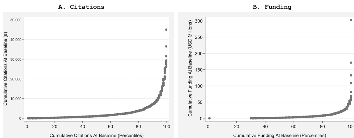
Fig. 7. Cumulative citations and funding at baseline. Note: We compute the cumulative number of citations (Panel A), and cumulative amount of funding (Panel B) up to the year preceding the corresponding earliest retraction event for all 376 retracted and 759 control authors, and plot it against 100 percentiles of the corresponding distribution.
