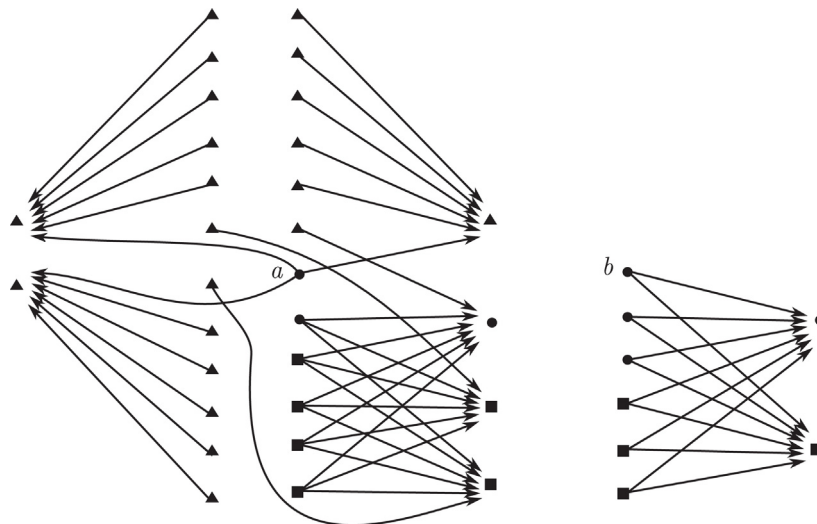
Fig. 4. Step 2. The network N_2 = (X_2, D_2) . The nodes added during step 2 (3 groups of 7 nodes) are represented by a triangle.
