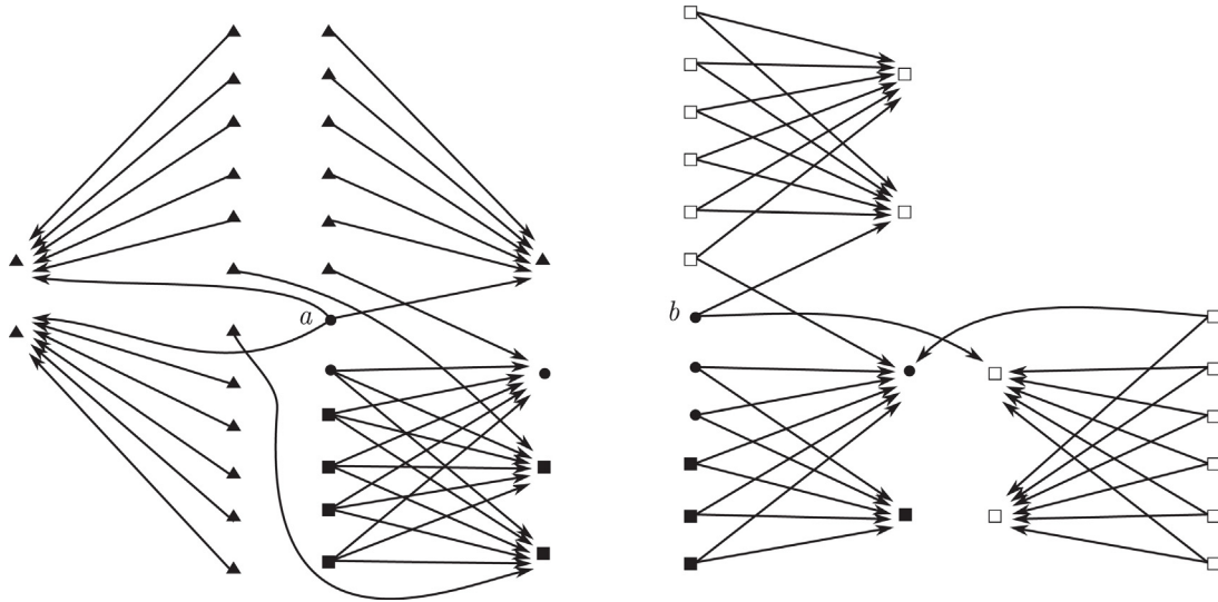
Fig. 5. Step 3. The network N_3 = (X_3, D_3) . The nodes added during step 3 (2 groups of 7 nodes) are represented by a empty square.
