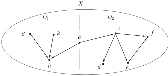
Fig. 7. Additivity. The network N=(X, D_1 \cup D_2) with two components connected via a .
