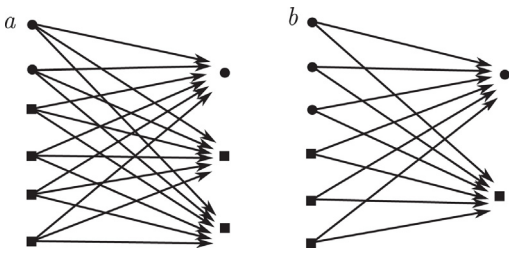
Fig. 3. Step 1. The network N_1 = (X_1, D_1) . The nodes added during step 1 are represented by a square. The least common multiple m is 6.
