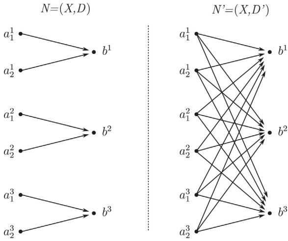
Fig. 1. Independence of Local Density: left, the network N=(X, D) and right, the network N'=(X, D') , with l=3 and n=2 .
