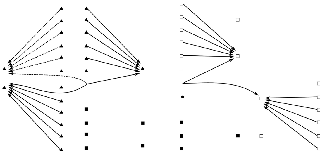
Fig. 6. Step 4. The network N_4 = (X_4, D_4) contains all arcs in this figure. The network N_5 = (X_5, D_5) contains only the solid arcs.
