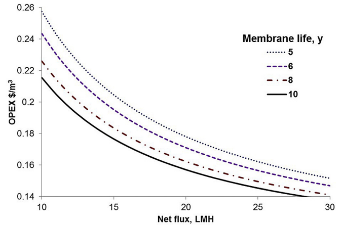
Fig. 3. MBR OPEX vs flux as a function of membrane life. SAD_m = 0.25 \text{ Nm}^3 \text{ m}^{-2} ; E_{L,m} = 0.015 \text{ kWh m}^{-3} ; L_m = \$25 \text{ m}^{-2} ; L_e = \$0.12 \text{ kWh}^{-1} ; \sum R = 5 ; E'_{A,m} = 0.022 \text{ kWh Nm}^{-3} ; E_{sludge} = 0.018 ; E'_{A,bio} SAD_{bio} = 0.5 \text{ kWh m}^{-3} .
