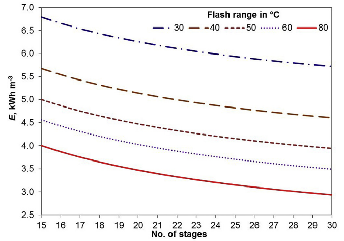
Fig. 1. Specific energy demand vs. number of stages at different flash ranges for an MSF.
