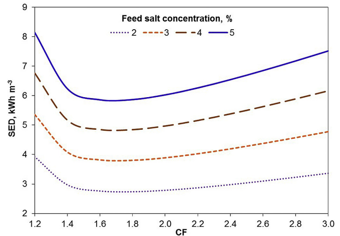
Fig. 2. Specific energy demand vs. brine concentration factor at different feed salt concentrations.
