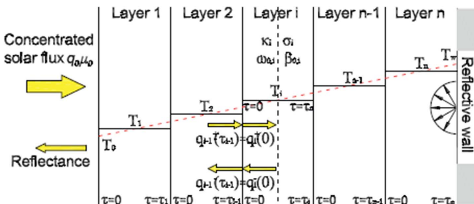
Fig. 14. Schematic of a multi-layer solar particle receiver [69].
