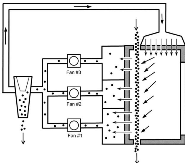
Fig. 10. Suction recirculation receiver [58].
