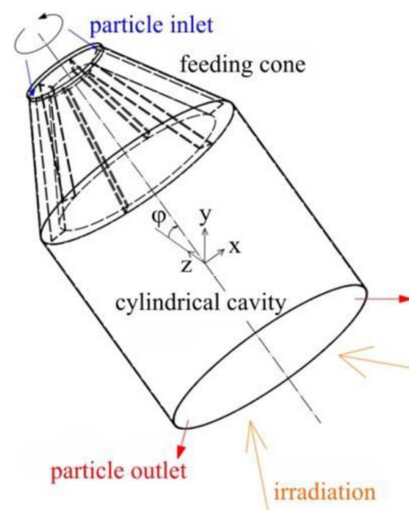
Fig. 9. Rotary kiln/centrifugal particle receiver [40].
