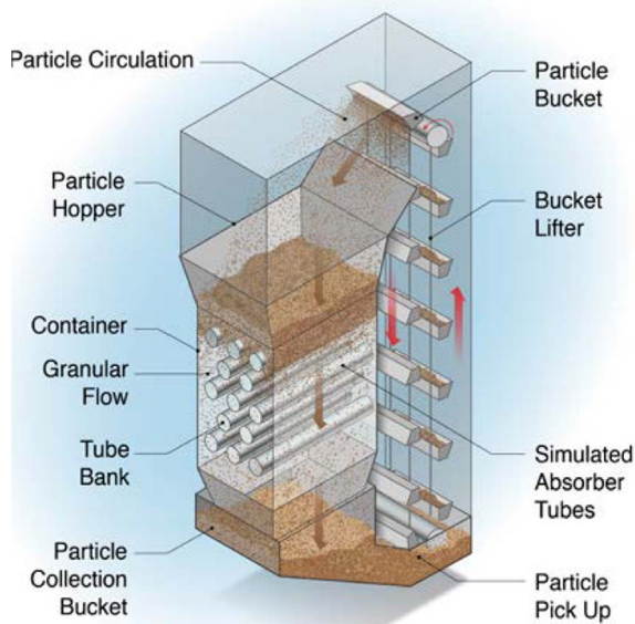
Fig. 12. Particle flow with HEX receiver [36].
