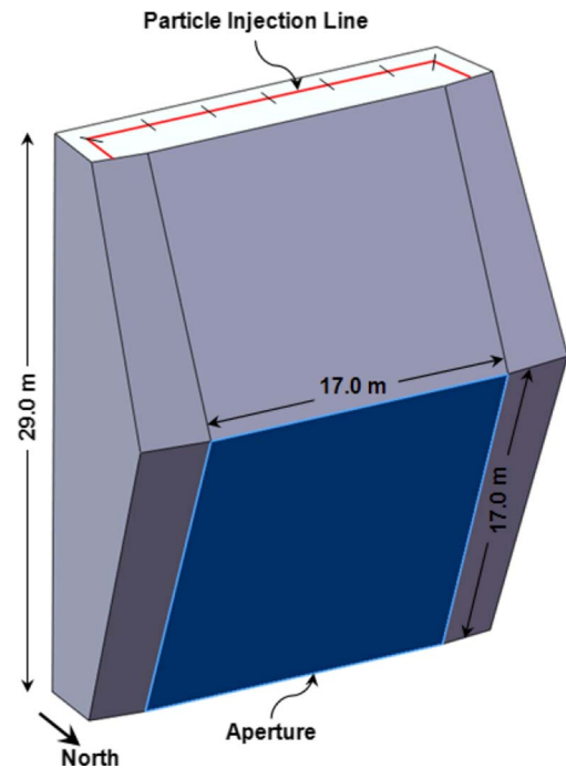
Fig. 5. Geometry of particle receiver [20].
