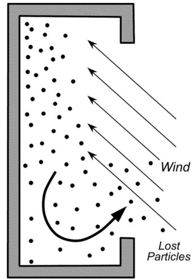
Fig. 11. Wind effect on the receiver [58].
