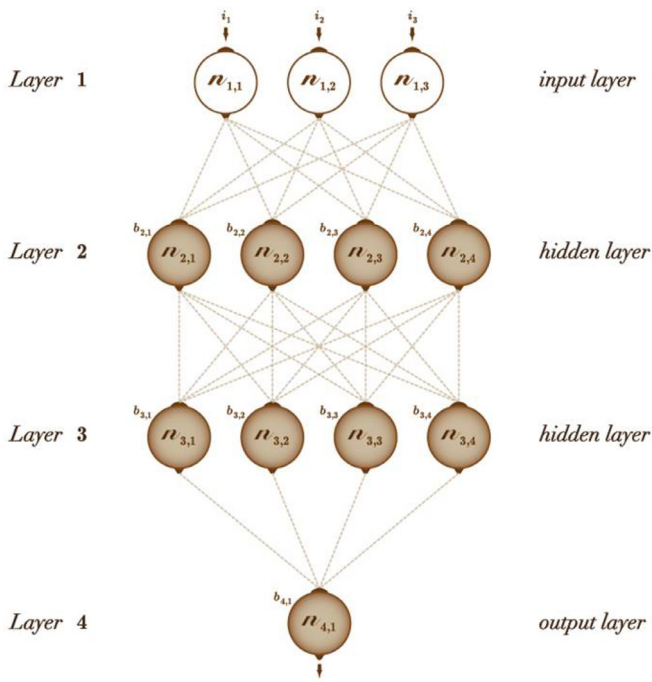
Fig. 2. Traditional ANN.
