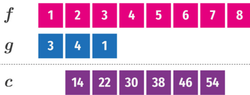
Fig. 5. Convolution layer.
