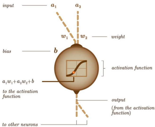
Fig. 3. Neuron structure.
