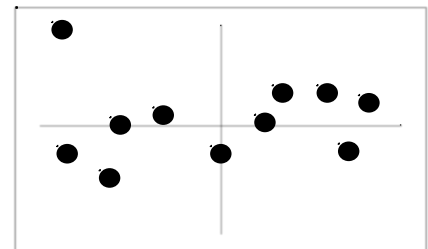
Software Engineering [11]
